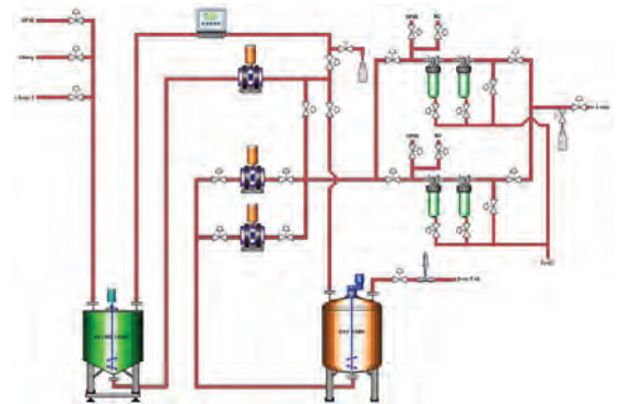
Configuration showing one blend tank, one day tank, redundant dispense pump, dispense filtration, and stirrer devices
